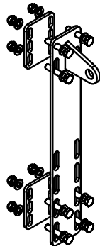
Top fixing bracket Span between steps: 250\text{mm} < e < 400\text{mm}
