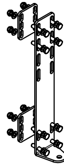
Low fixing bracket Span between steps: 250\text{mm} < e < 400\text{mm}
